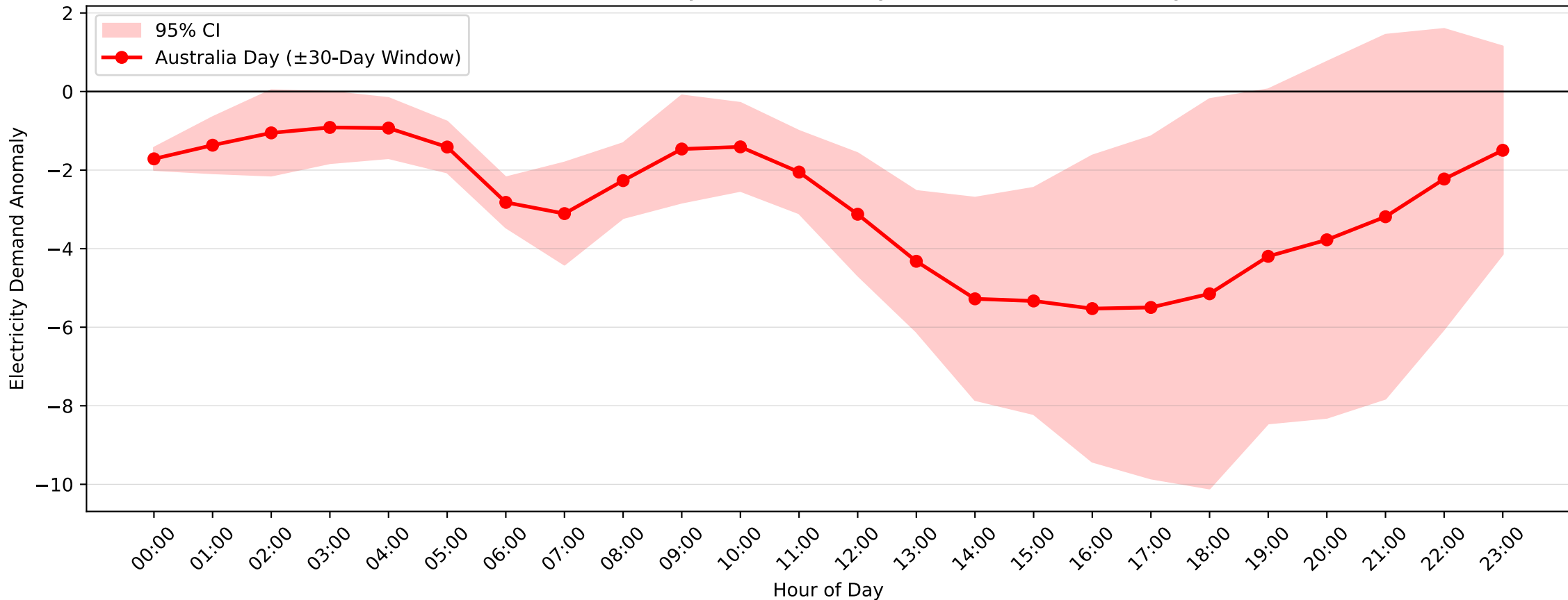
Mortdale Demand Anomaly: Australia Day (2016–2017, \pm 30 -Day Window)
